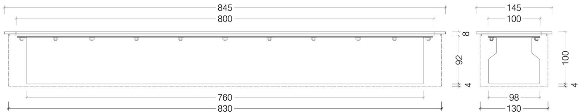
Front View
