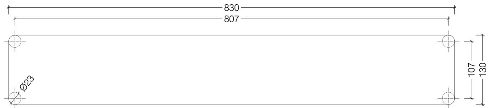
Front View
