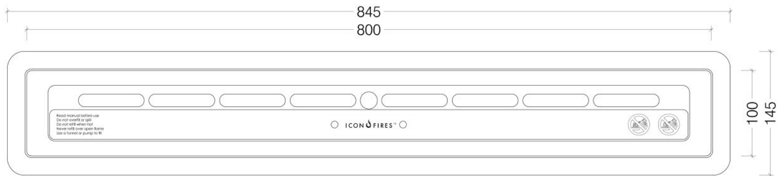
Top View
