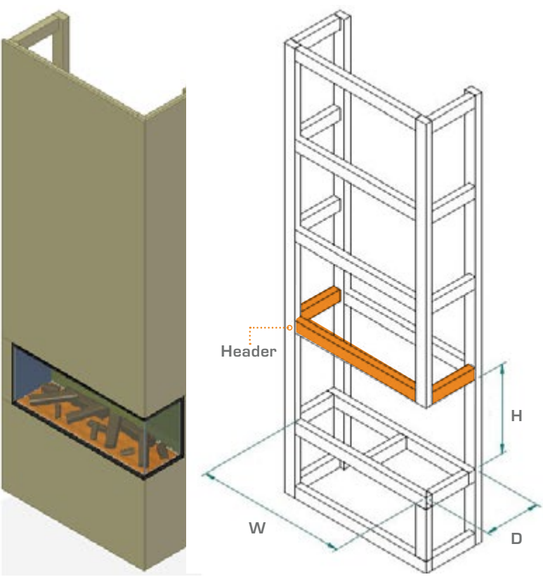
// Two-sided installation
