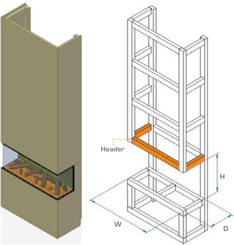
// Three-sided installation
